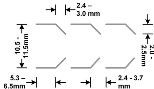
Figure 12- Zip Tie Dimensions (not to Scale):
